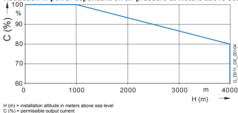
Reduction in power dependent on air pressure at meters above sea level
