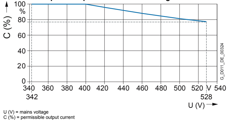
Reduction in power dependent on mains voltage
